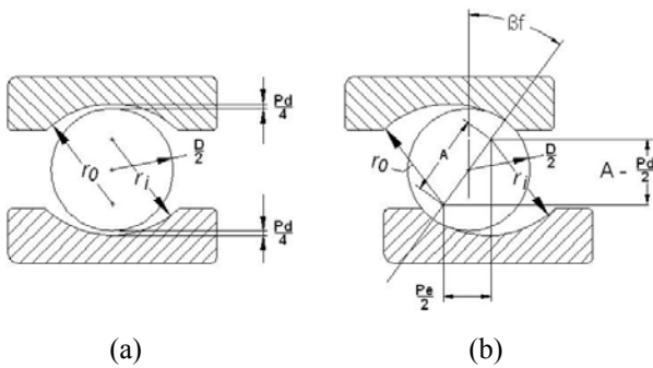
Fig. 4 Cross section of a radial ball bearing showing ball-race contact due to axial shift of inner and outer rings. (a) Initial position. (b) Shifted position
