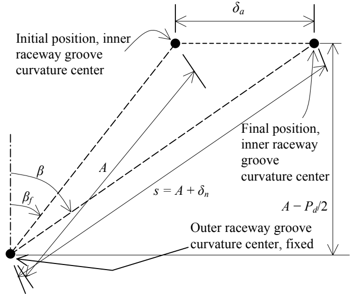
Fig. 7 Positions of ball center and raceway groove curvature centers at angular position \psi , with and without applied load
