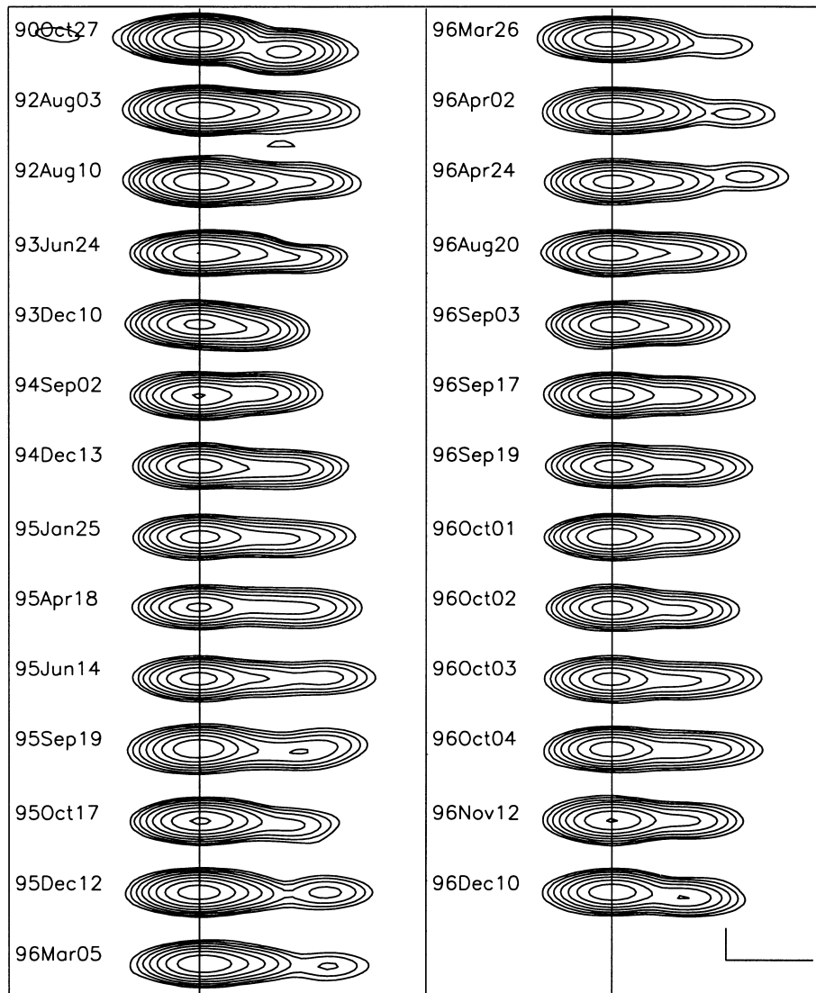
FIG. 1.—8 GHz VLBI maps of OJ 287. Contour levels increase as 2^\circ . The lowest contour level is 0.01 \text{ Jy beam}^{-1} , corresponding to n = 0 . The restored circular beam is 0.6 mas. The stationary component (the VLBI core) is on the east side (left), while the moving components are to the west (right). The tick in the lower part of the map indicates the size in mas. Note that the maps are stretched in right ascension.
