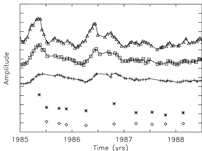
FIG. 5.—Radio light curves compared to VLBI light curves from Vicente et al. (1996). Below the radio light curves are shown the flux of the core (asterisks) and the sum of the flux of the jet components (diamonds) from Vicente et al. (1996). All amplitudes are on the same scale. Each tick mark on the ordinate corresponds to a flux density of 2 Jy.
