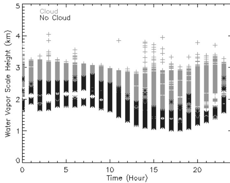
Figure 4 Water vapour scale height in km versus time in hrs by radiometry at INPE, Brazil (January, 2009).
