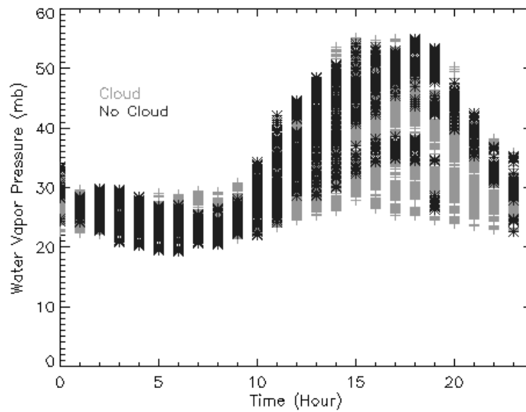
Figure 2 Water vapour pressure in mb versus time in hrs by radiometry at INPE, Brazil (January 2009).
