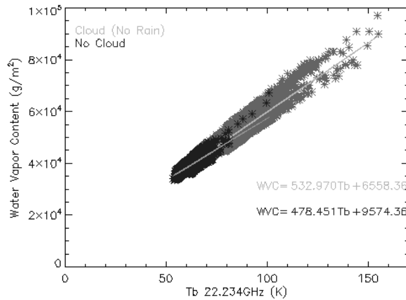
Figure 5 Water vapour content ( \text{g/m}^2 ) versus brightness temperature in Kelvin at 22.234 GHz by radiometry at INPE, Brazil (Jan 2009).
