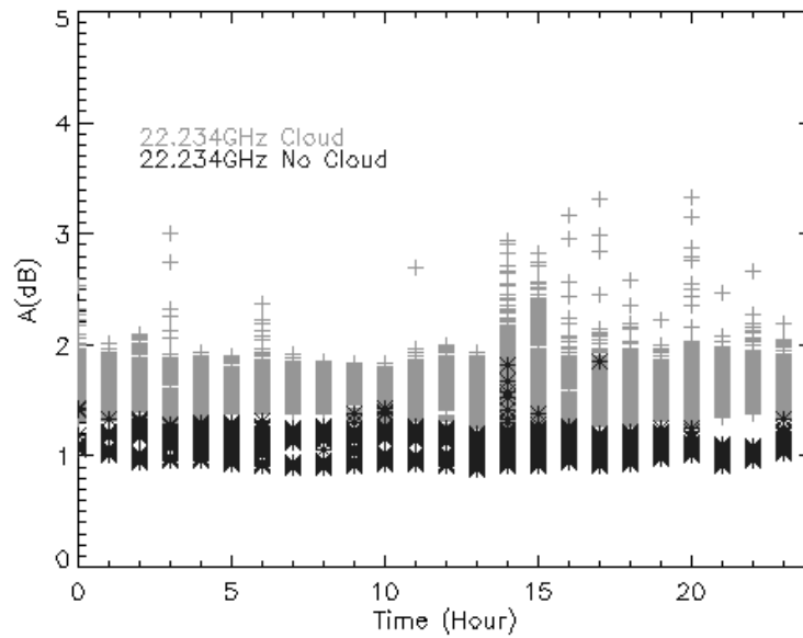
Figure 1. Radiometric attenuation at 22.234 GHz at INPE, Brazil, during January 2009.
