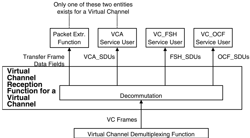
Figure 4-14: Abstract Model of Virtual Channel Reception Function
