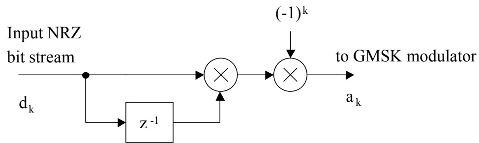
Figure 2.4.18-1: GMSK Precoder
