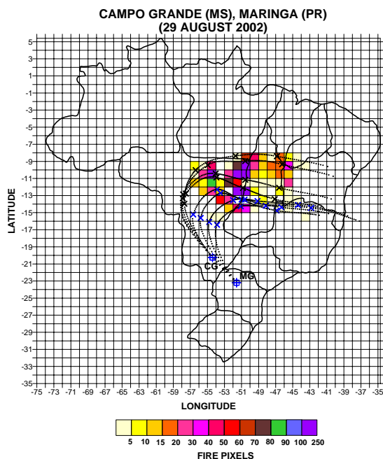
Fig. 5 – Five day backward trajectories from Campo Grande (20°S; 54°W) and Maringá (23.1°S; 53.1°W) and the fire pixels along the path. The crosses show one day along the path.
