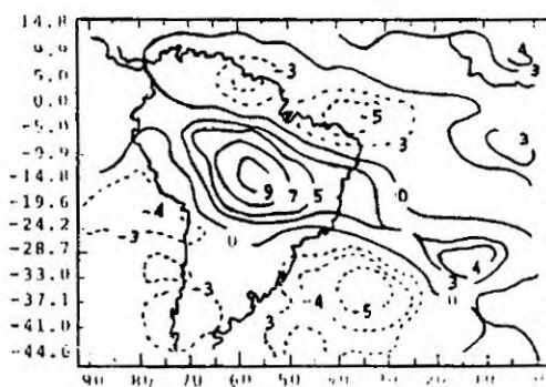
Fig. 2: Matriz-Correlation between BH and SACZ
