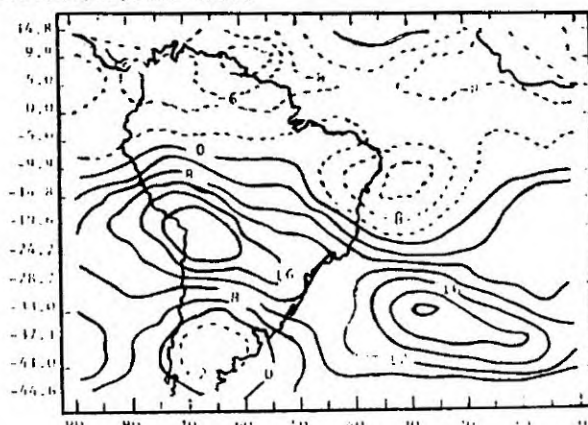
Fig. 1: Ten-year-average Relative Vorticity for January
