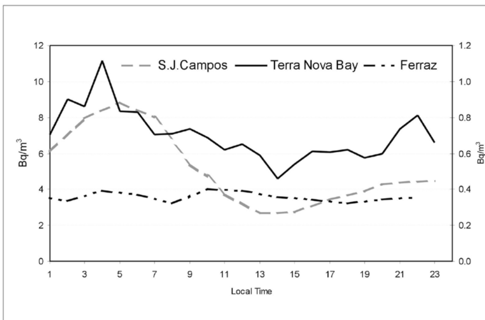
Figure 6 - Daily concentration profile of radon in Terra Nova as compared to profiles obtained with the same technique in sites located at higher latitudes. Values on the principal Y axis on the left are referred to data collected in S.Josè dos Campos, while the secondary Y axis is referred to Antarctic data (Terra Nova Bay and Ferraz).
