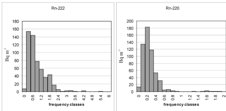
Fig.3 – Frequency distribution of 222 Rn and 220 Rn
