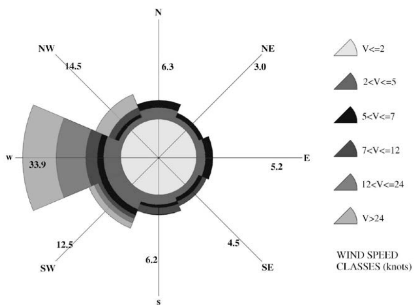
Fig.8 – Rose wind for the Automated Weather Station Eneide at Terra Nova Bay.
