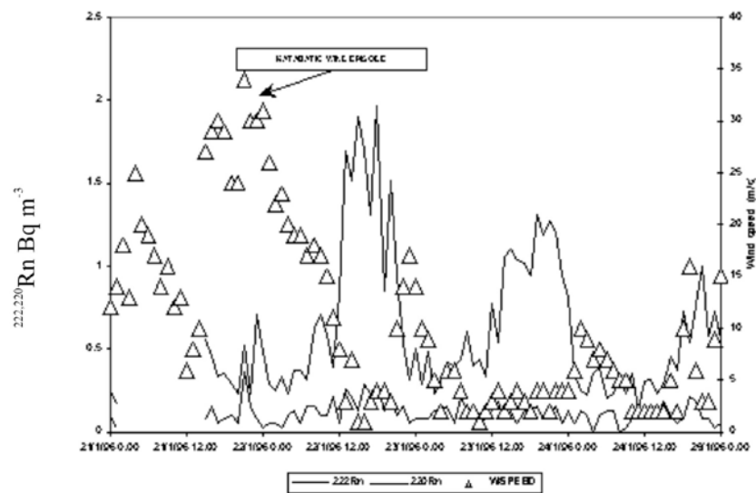
Fig.4 - Effect of katabatic winds on radon concentration at Terra Nova Bay, episode recorded during the 1995-96 summer campaign.
