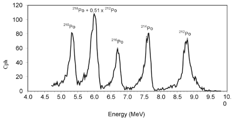
Fig. 2 – Alpha spectrum of ^{222,220}\text{Rn} progeny obtained with the electrostatic precipitator built at INPE.
