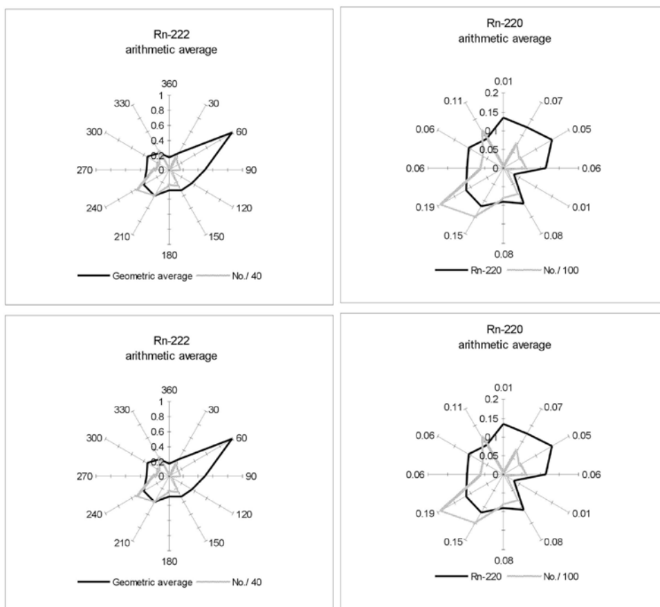
Fig. 7 – Radar diagrams for ^{222}\text{Rn} , ^{220}\text{Rn} activities and frequencies in association with geographical origin. Radon data refer to 1997-98 summer campaign.
