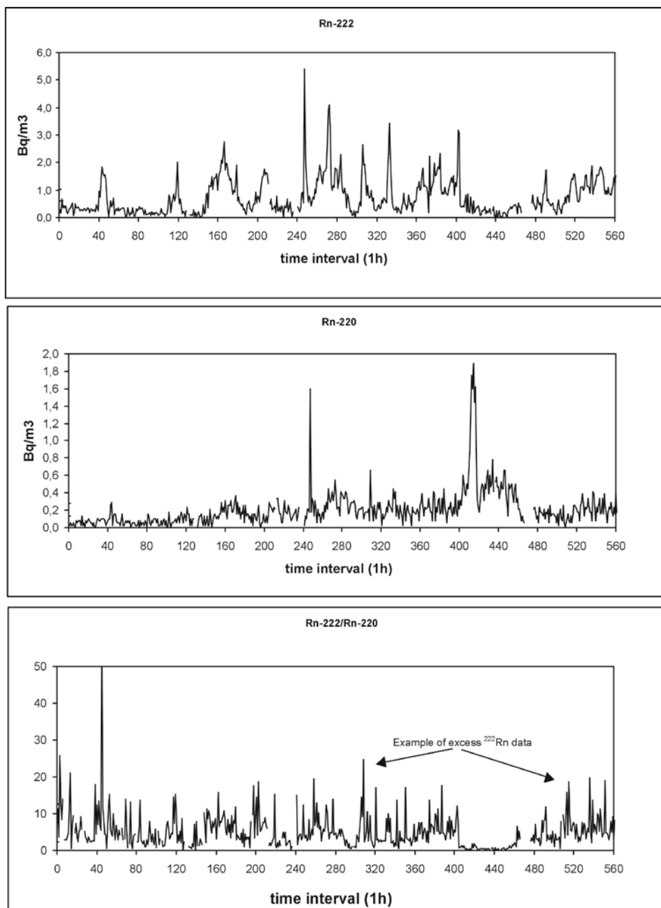
Fig. 5 - ^{222}\text{Rn} , ^{220}\text{Rn} , ^{222}\text{Rn}/^{220}\text{Rn} ratio time-series in 1997-98 summer expedition. In the diagram excess ^{222}\text{Rn} values and consequent highest isotopic ratios are highlighted.
