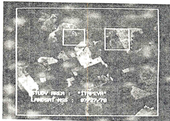
Figure 2 - Location of the study sites for forest of eucalyptus (LANDSAT MSS-5).
