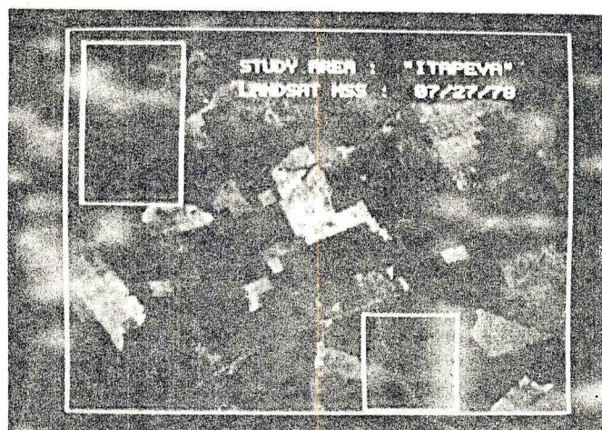
Figure 4 - Location of the study sites for vegetation of "cerrado" (LANDSAT MSS-5).
