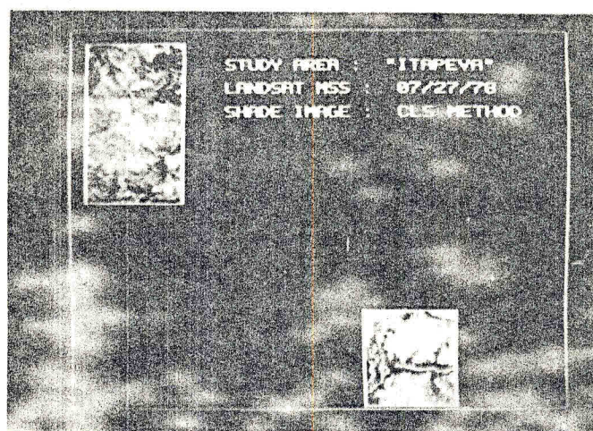
Figure 5 - Shade images for vegetation of "cerrado".
