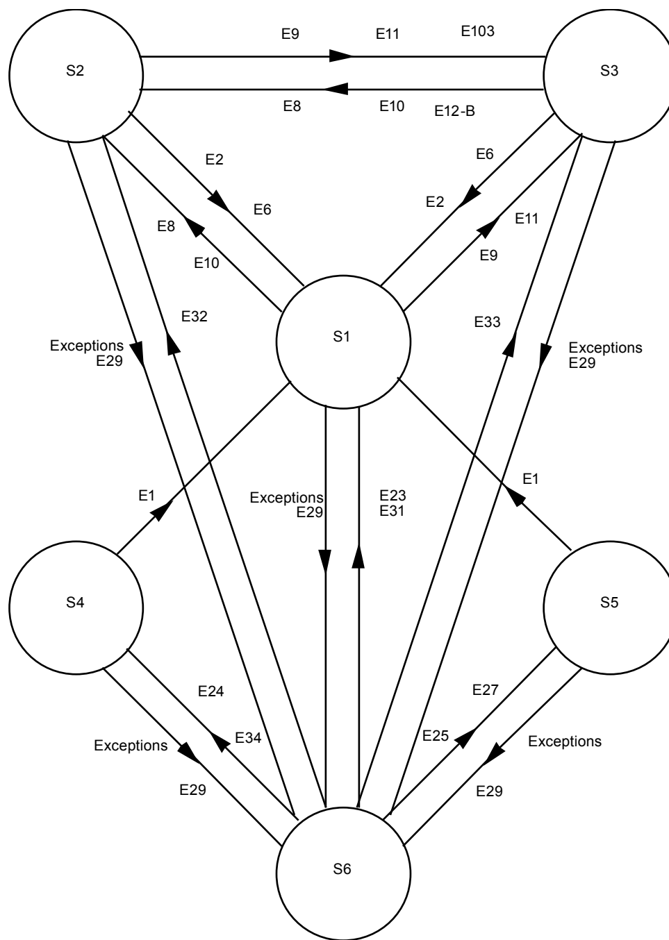
Figure 5-3: FOP-1 State Transitions
