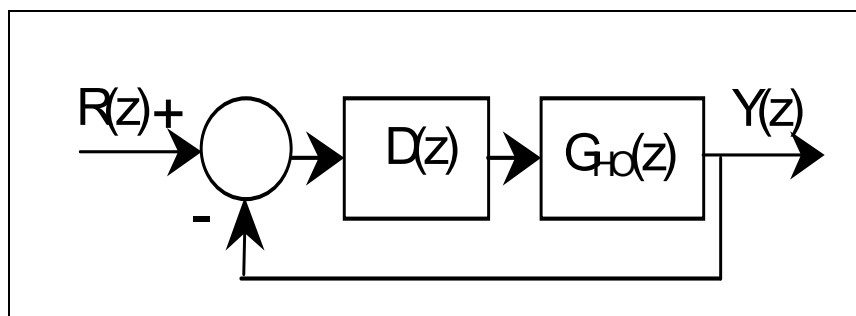
Fig.6: Discrete-time approximation to the closed-loop analog control system.
