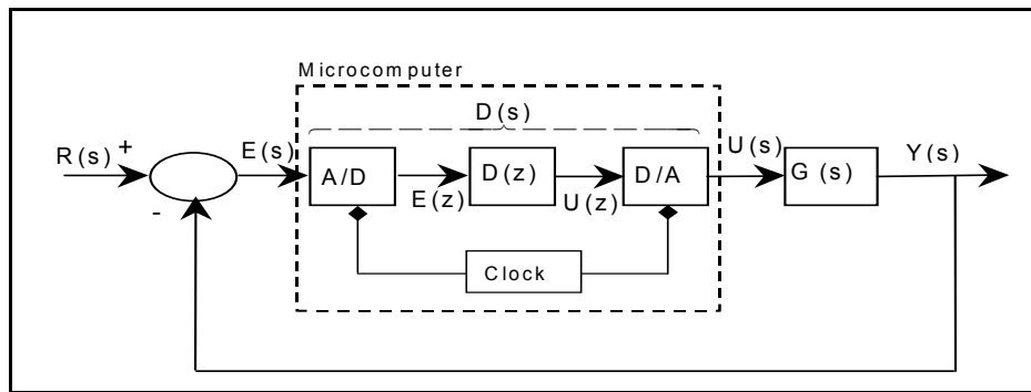
Fig.3: Closed-loop digital control system rearranged (1).
