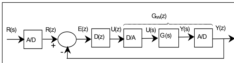
Fig.4: Closed-loop digital control system rearranged (2).
