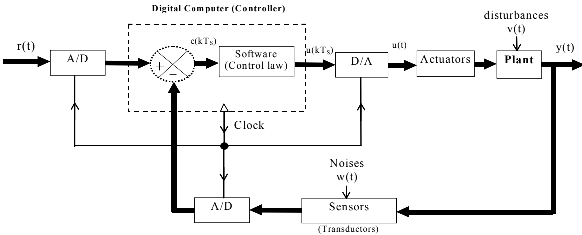
Figure 2: Closed-loop digital control system block diagram.
