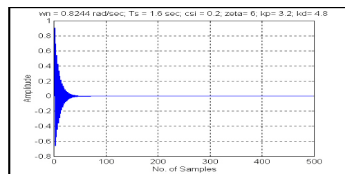
Fig. 10. Overdamped harmonic oscillator controlled by a PD designed by the new-rule ( T_s = 1,6 seconds): assymptot.stable.
