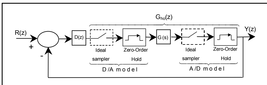
Fig.5: Closed-loop digital control system rearranged (3) with A/D and D/A sample & hold models.
