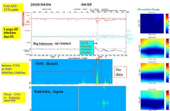
Fig.5 AE index, CNA Keogram at SSO and Kakioka. Right side images are CNA at SSO when GALAXY-15 is breakdown.
