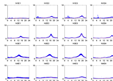
Fig.3 QDC at Concepcion (Chile) in 2007/05 (one month)
